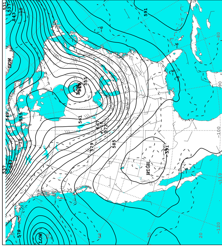
500-Millibar Height Contours at 7:00 A.M. E.S.T.
