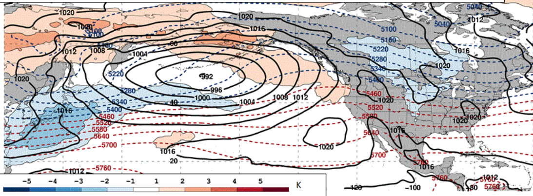
Mean Sea-Level Pressure, 1000–500-hPa Thickness, 850-hPa Temp. Anomalies: Day 0
